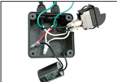
Figure 20. Switch connections.
